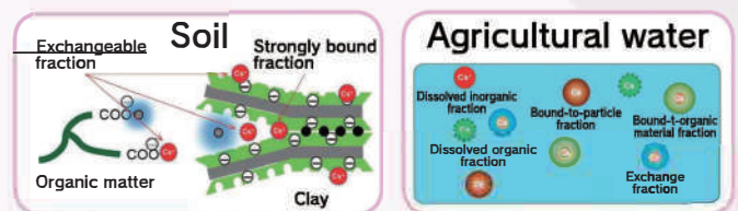
(FIG) Chemical speciation of radiocaesium in soil and irrigation water
