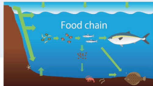
Overview of biogeochemical cycles
